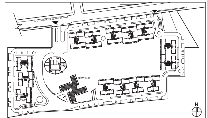
SITE PLAN
